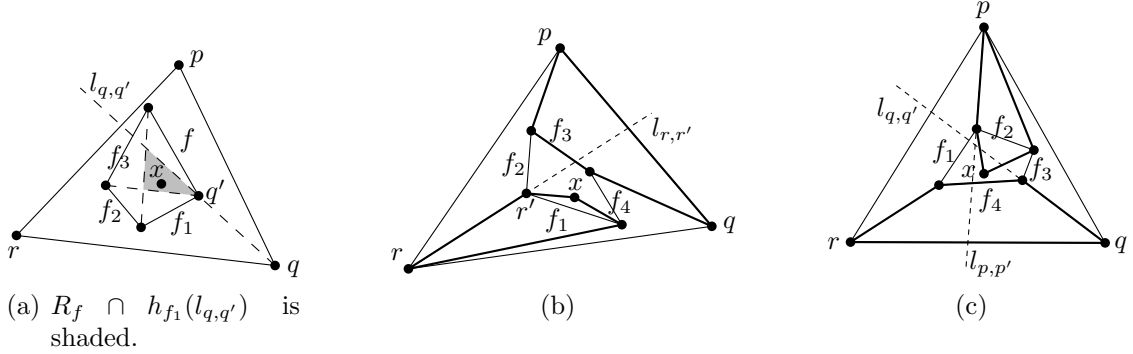
Fig. 11. |H| = 3 , |H'| = 4 .
