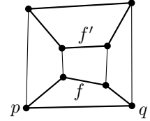
Fig. 8. |H| = 4 , |H'| = 4 .
