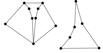
Fig. 2. Sets with non-monotone behavior.
