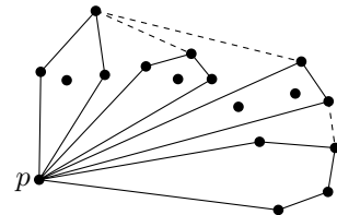
Fig. 4. Petals of size 5.
