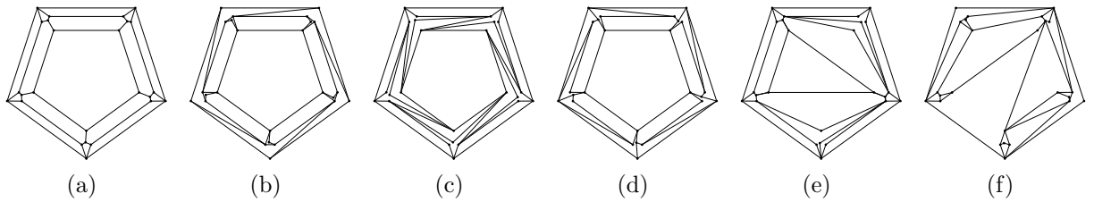
Fig. 17. Five tilings of the convex hull of S_5 with 16 convex or pseudo-triangle faces (a–e), and one with 17 faces (f).
