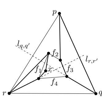
Fig. 12. |H| = 3 , |H'| = 4 .
