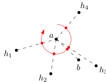
Fig. 1. A point set with R_\chi(a) = h_4, h_3, b, h_2, h_1 .
