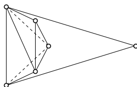
Figure 3: The greedy pointed pseudo-triangulation (solid) differs from the MWPT (dashed).
